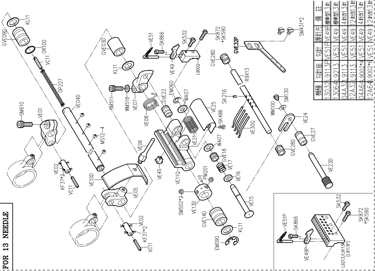
FOR 13 NEEDLE
